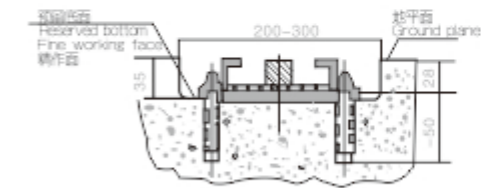
埋入地面式轨道组断面图 Sectional drawing of buried track group
