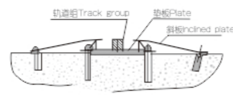
斜板地面式轨道组断面图 Sectional drawing of inclined plate ground track group
